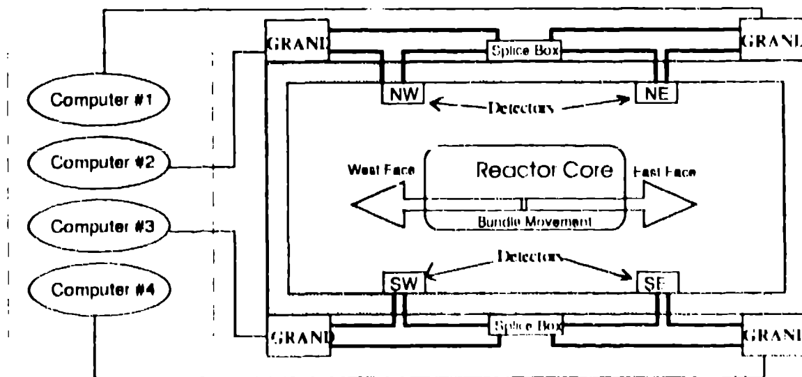
Fig. 2. Sample layout of a typical on load reactor
